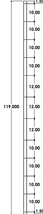
MODEL CH5LS-119.00" (10'0") SHOWN FOR EXAMPLE
