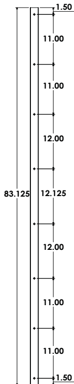
MODEL CH5LS-83.125" (7'0") SHOWN FOR EXAMPLE
