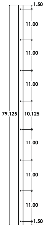
MODEL CH5LS-79.125" (6'8") SHOWN FOR EXAMPLE
