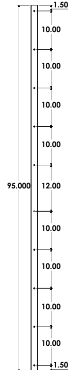
MODEL CH5LS-95.000" (8'0") SHOWN FOR EXAMPLE
