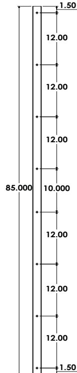
MODEL CH5LS-85.000" (7'2") SHOWN FOR EXAMPLE
